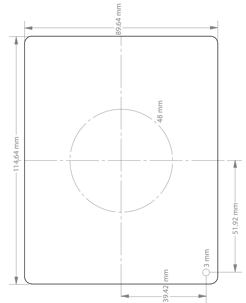
Figure 2 Truecharge2 Remote Panel Mounting Template (1:1)
